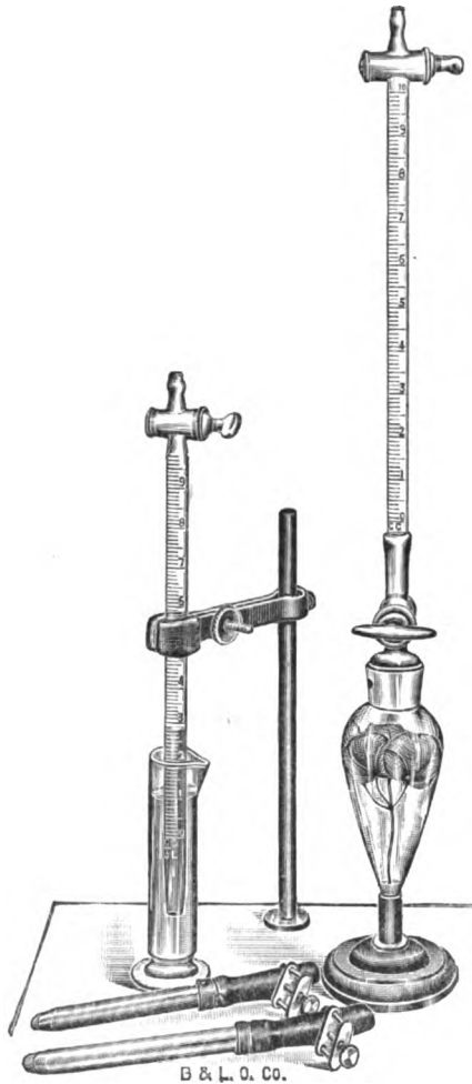
FIG. 7.—A photosynthometer, by which the gas exchange in photosynthesis is quantitatively tested; \times \frac{1}{2} .
